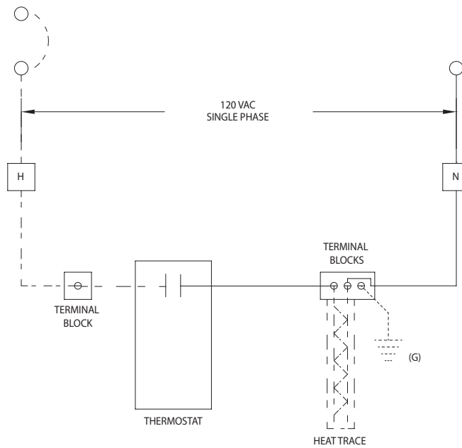
SHOWER CONTROL WIRING SCHEMATIC CIRCUIT BREAKER WITH GFCI REQUIRED (FOLLOW NEC AND LOCAL ELECTRICAL CODES)
