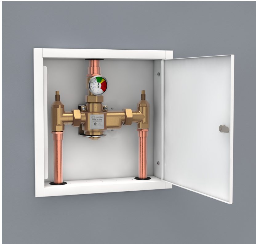
Unit shown is G6043.1R1
